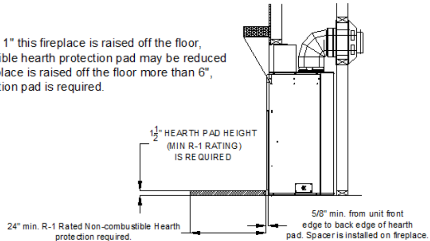
Figure 3-9HEARTH PAD GUIDE
