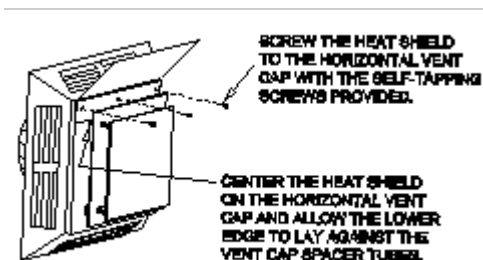
Figure 3-14 WALL HEAT SHIELD
