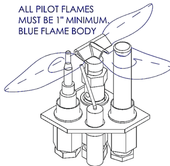
Figure 4-9 Pilot Flames
