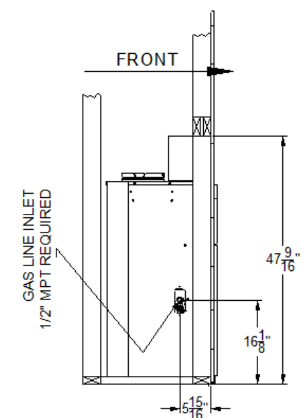
Figure 3-19 Gas Line Inlet Location
