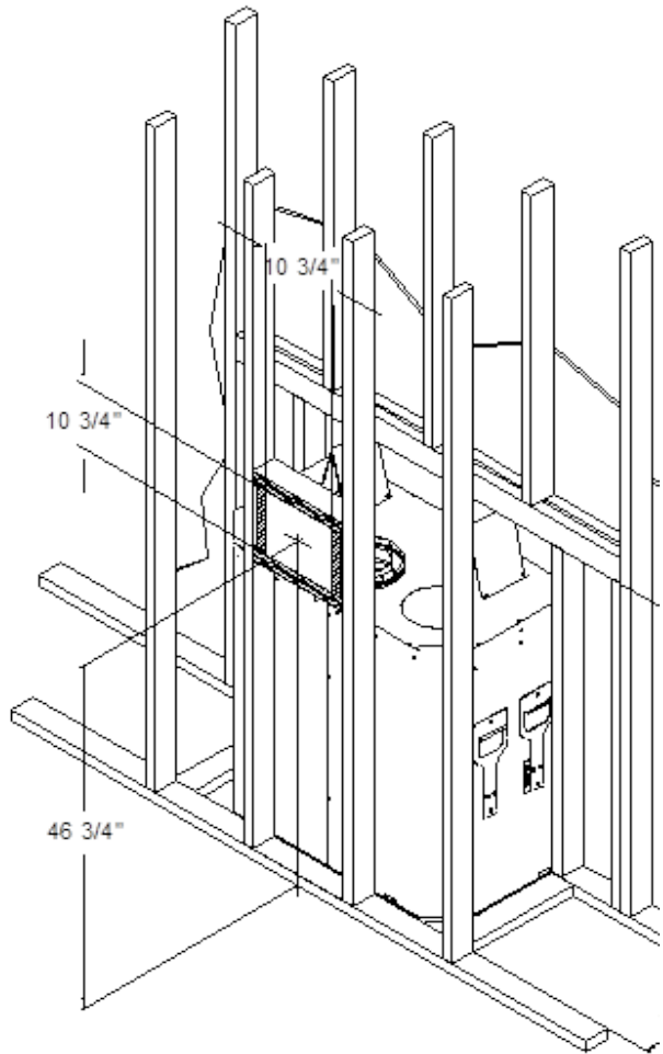
Figure 3-4 FRAMING METHOD
