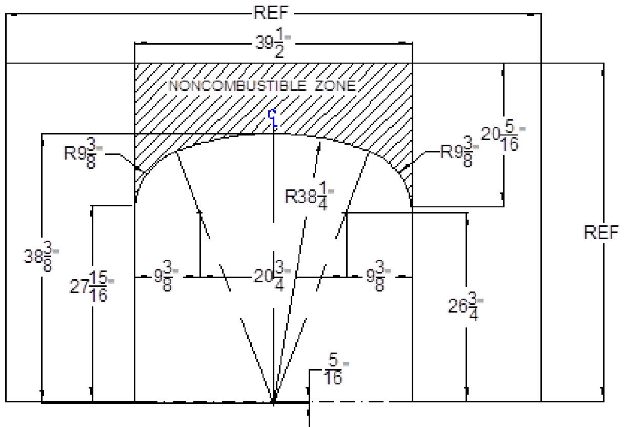
Figure 3-13 FINISHING MATERIALS CUTTING DIMENSIONS
