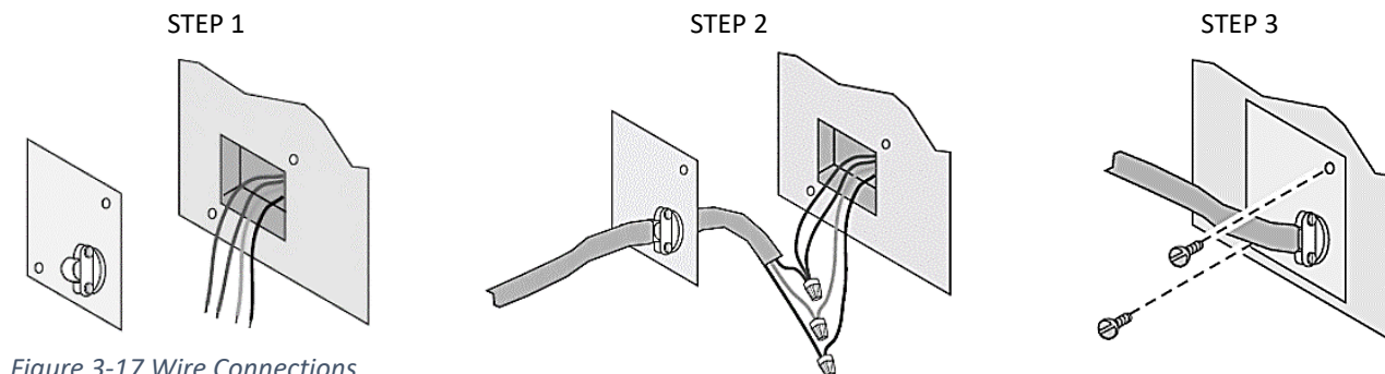
Figure 3-17 Wire Connections
