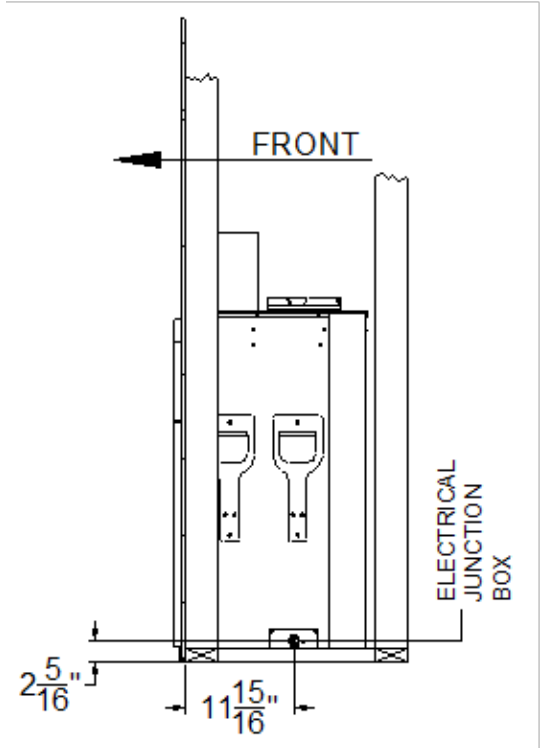
Figure 3-16 Electrical Junction Box
